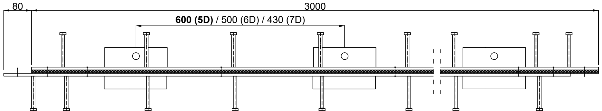
Conecto Dowel 08NA40-5D-T8 h=175 PC L=3000, black steel, with foam 10mm
