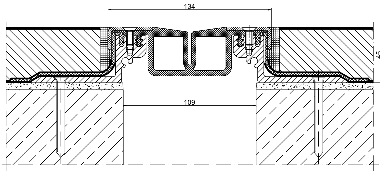
CONECTO GA 88.45.45 L SECTION
