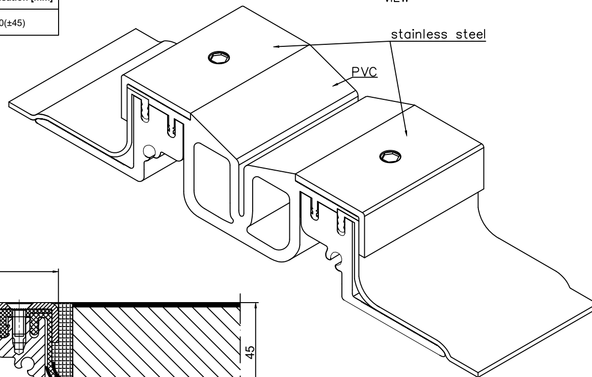
CONECTO GA 88.45.45 L VIEW
