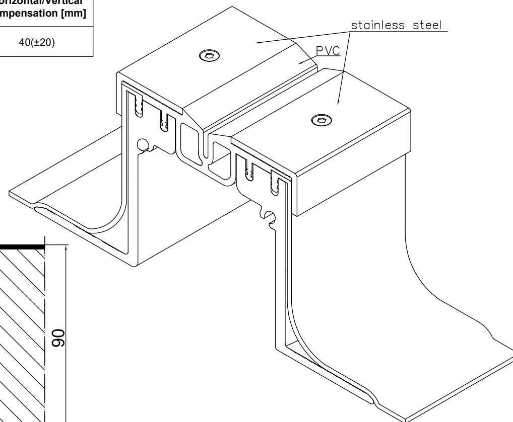
CONECTO GA 50.20.90 L VIEW
