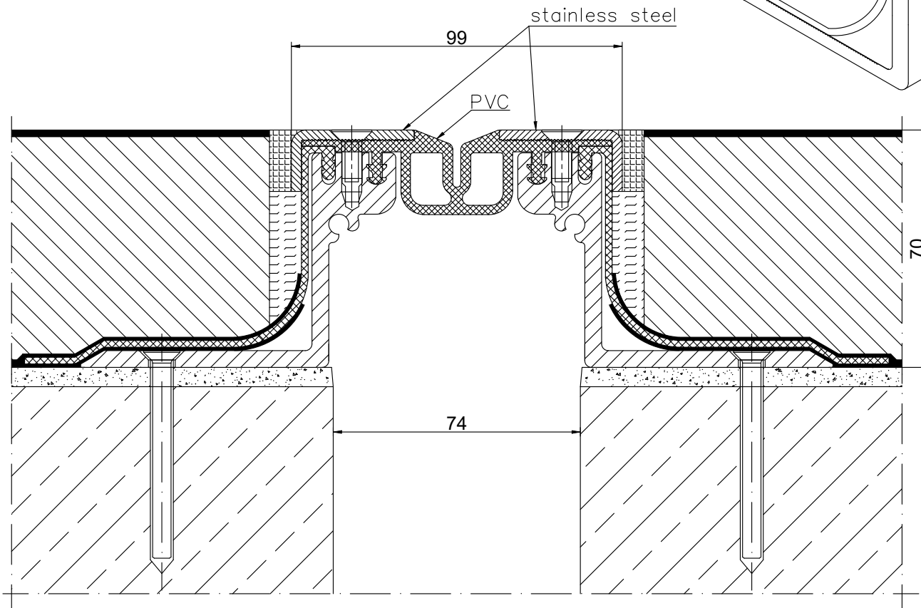
CONECTO GA 50.20.70 L SECTION
