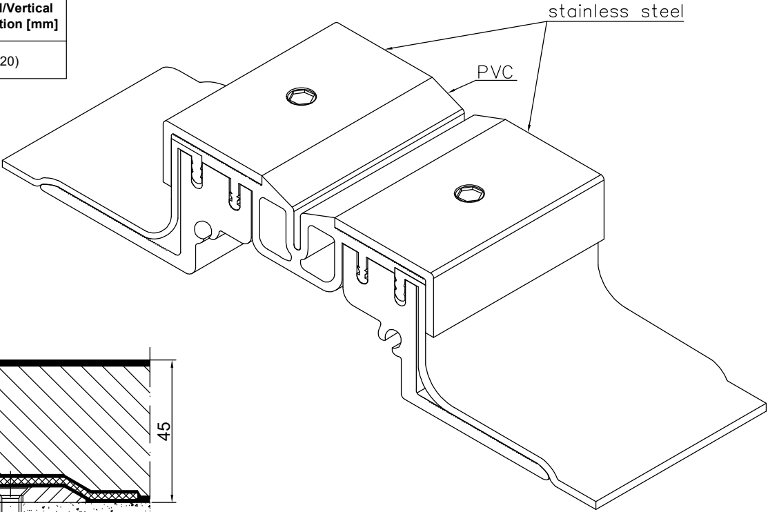
CONECTO GA 50.20.45 L VIEW
