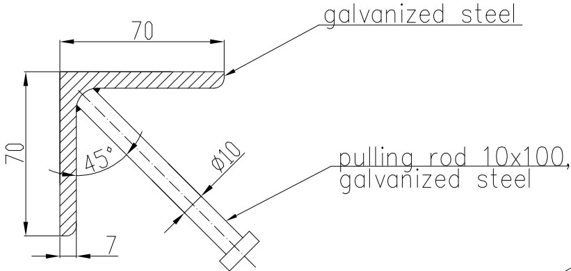
Angle 70x70x7 reinforced galvanized steel Section Scale 2:1
