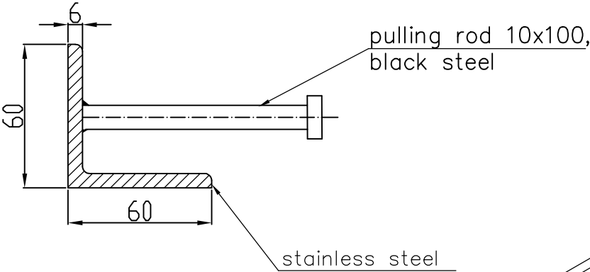
Angle 60x60x6 reinforced stainless steel Section Scale 2:1
