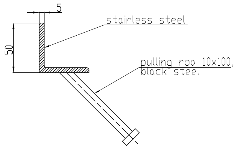
Angle 50x50x5 reinforced stainless steel Section Scale 2:1
