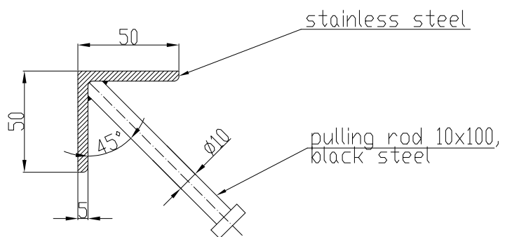
Angle 50x50x5 reinforced stainless steel Section Scale 2:1
