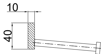
Conecto Single Strip Joint 10NA40 Section
