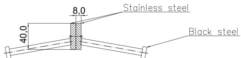
DOUBLE STRIP JOINT 08NA40 reinforced Section
