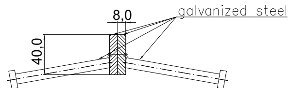
DOUBLE STRIP JOINT 08NA40 reinforced Section
