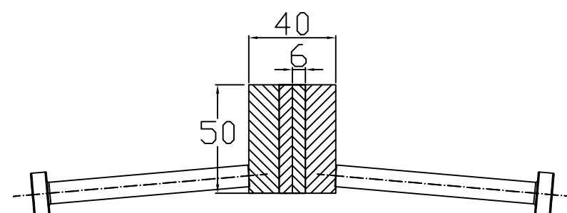
Conecto sinus 06NS50 reinforced SECTION
