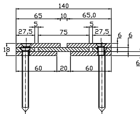
Conecto Sinus 06NC140/18-R S20K10 Section
