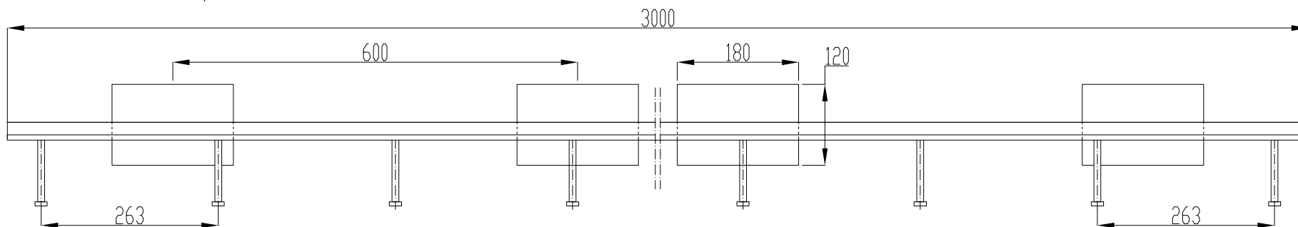
Conecto Omega 03NB-5D-T8 h=160/175 Top view scale 1:1,25
